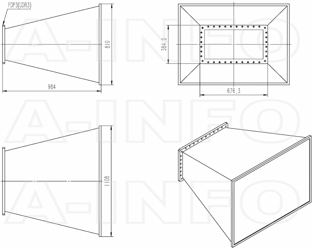
FDP3 Output with Radome (Option, P/N: LB-2300-10-ASPO, Outdoor Application)
