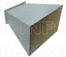
LB-2300-10-A Standard Gain Horn Antenna 0.32-0.49GHz 10dB Gain Rectangular Waveguide Interface
